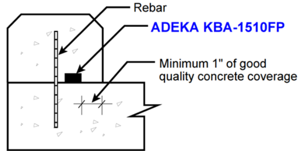
No Scale CONTAINMENT CURB
